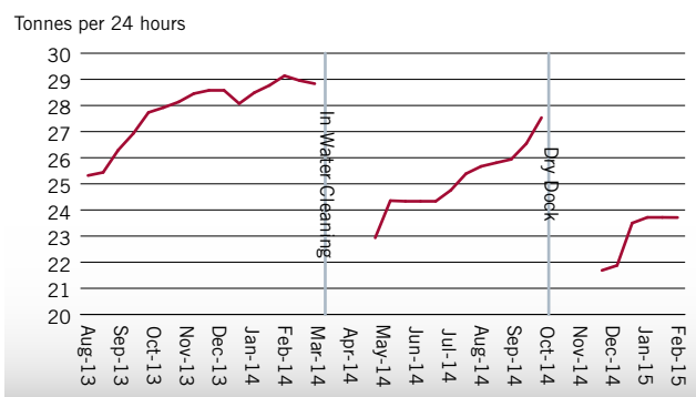
Cleaning of hull and propeller reduces the vessels' fuel consumption significantly.
